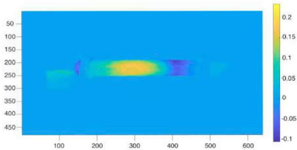
Fig. 1. Difference obtained from the subtraction of two thermal images where the pipe had different distribution of dust along it.
