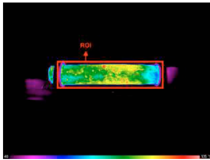
Fig. 5. Example of a thermal image obtained in the experiment when the duct had sediment inside.
